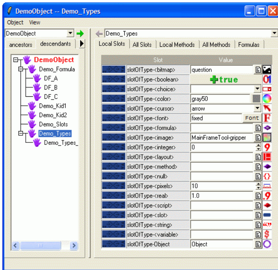
Figure 3: Object browser
